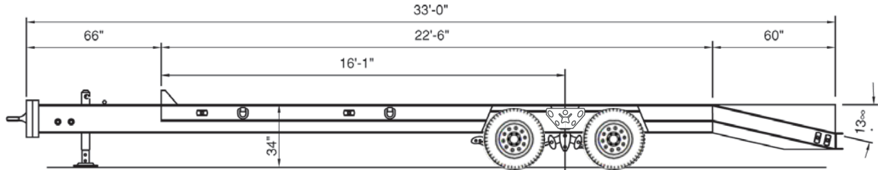
TANDEM AXLE MODEL SHOWN
